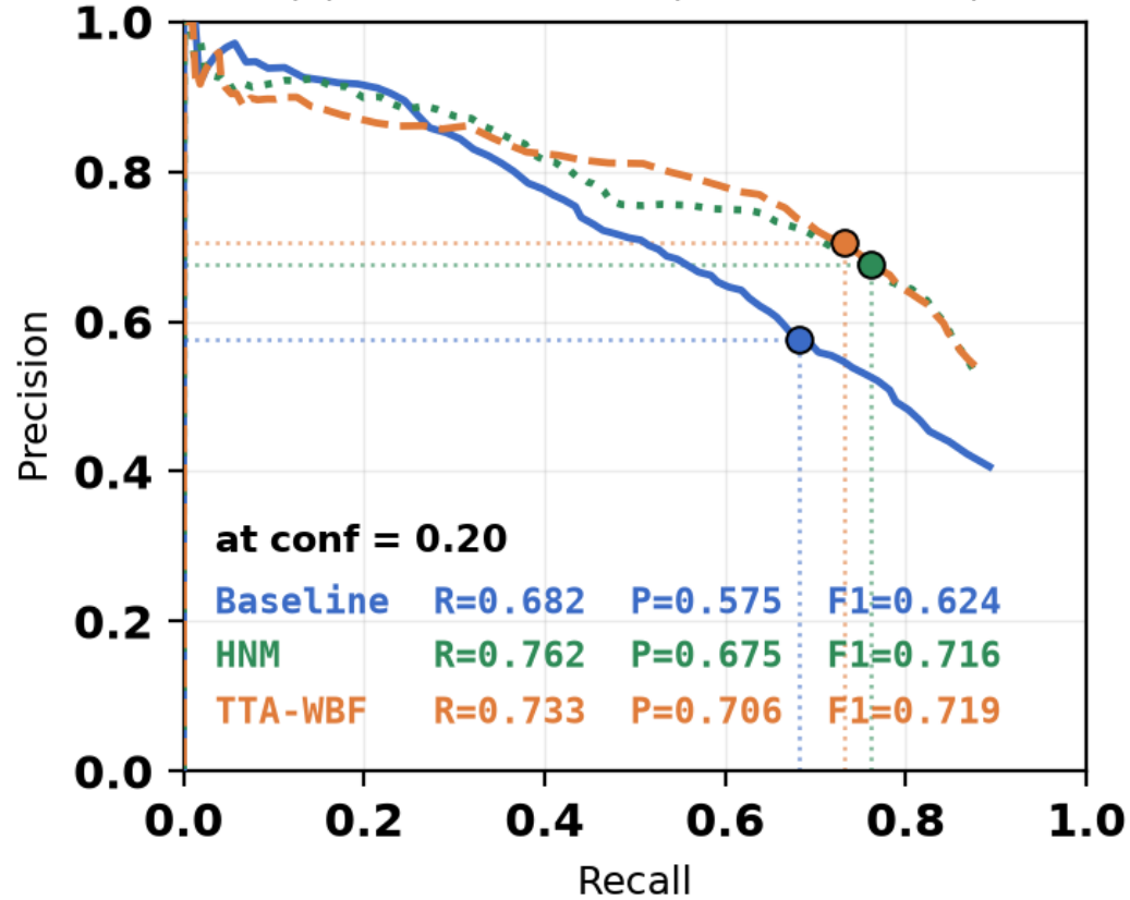
(a) Precision-Recall (conf 0.05-0.85)
