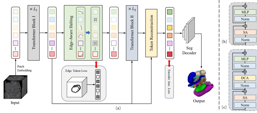
Fig. 1. Overview of the proposed HRViT for medical image segmentation. (b) Standard Transformer block ( TB_I ). (c) Transformer block with edge reinforcement ( TB_{II} ).
