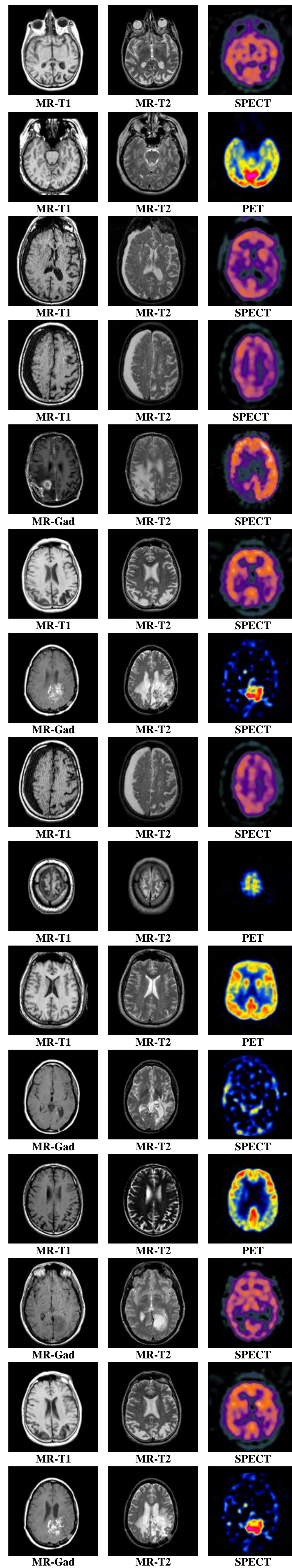
Ground Truth
