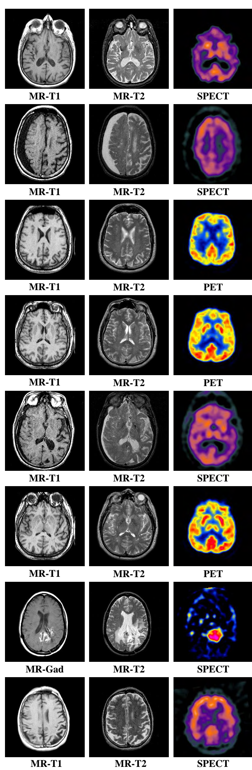
Ground Truth
