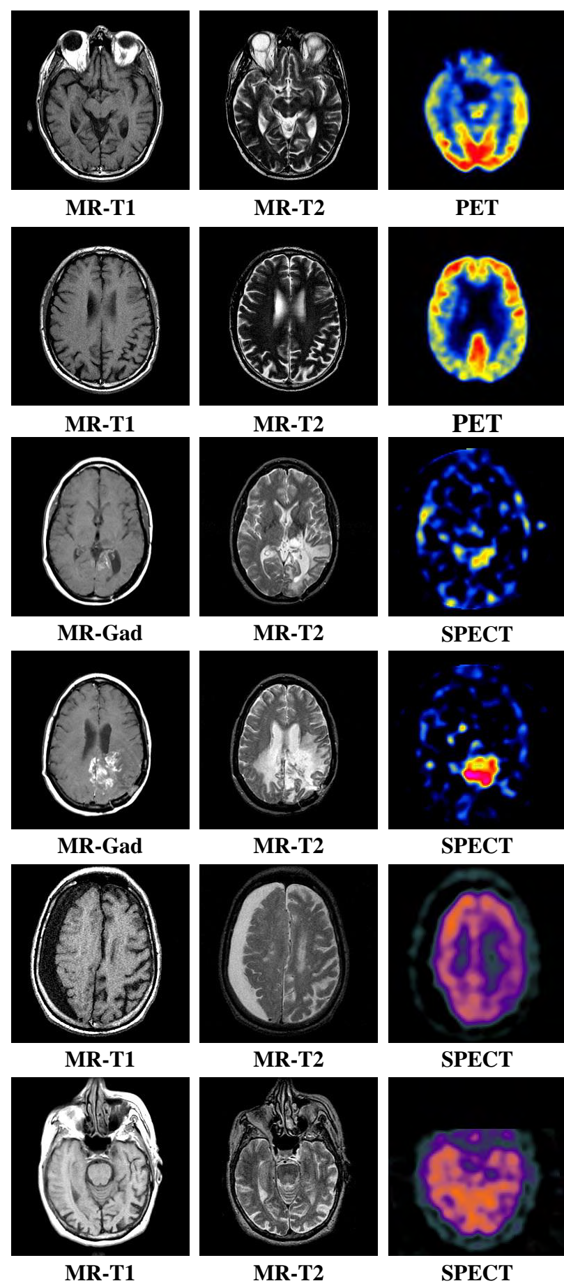
Ground Truth
