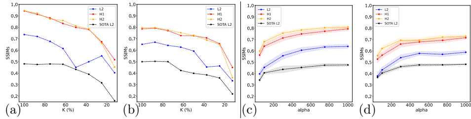
Fig. 1. Robustness of the proposed method. (a-b) SSIMs as a function of the number of measurement with known (Fig. 1a) and estimated motion (Fig. 1b). (c-d) SSIMs as a function of the noise level with known (Fig. 1c) and estimated motion (Fig. 1d). The shaded area represent the 95% confidence interval around the mean.
