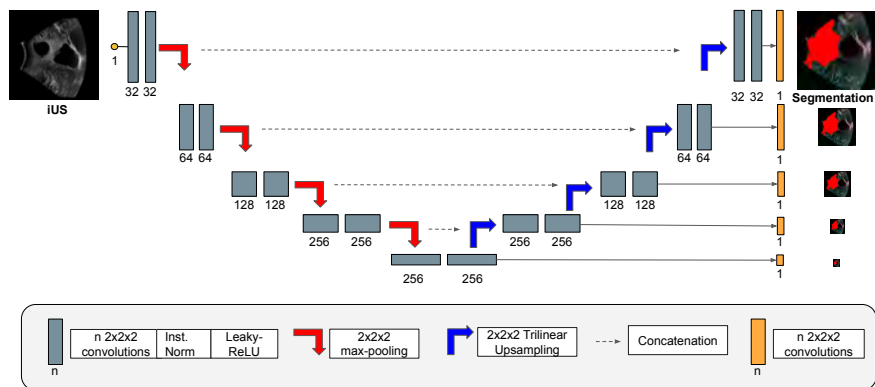
Fig. 2. Our 2D Unet segmentation network.
