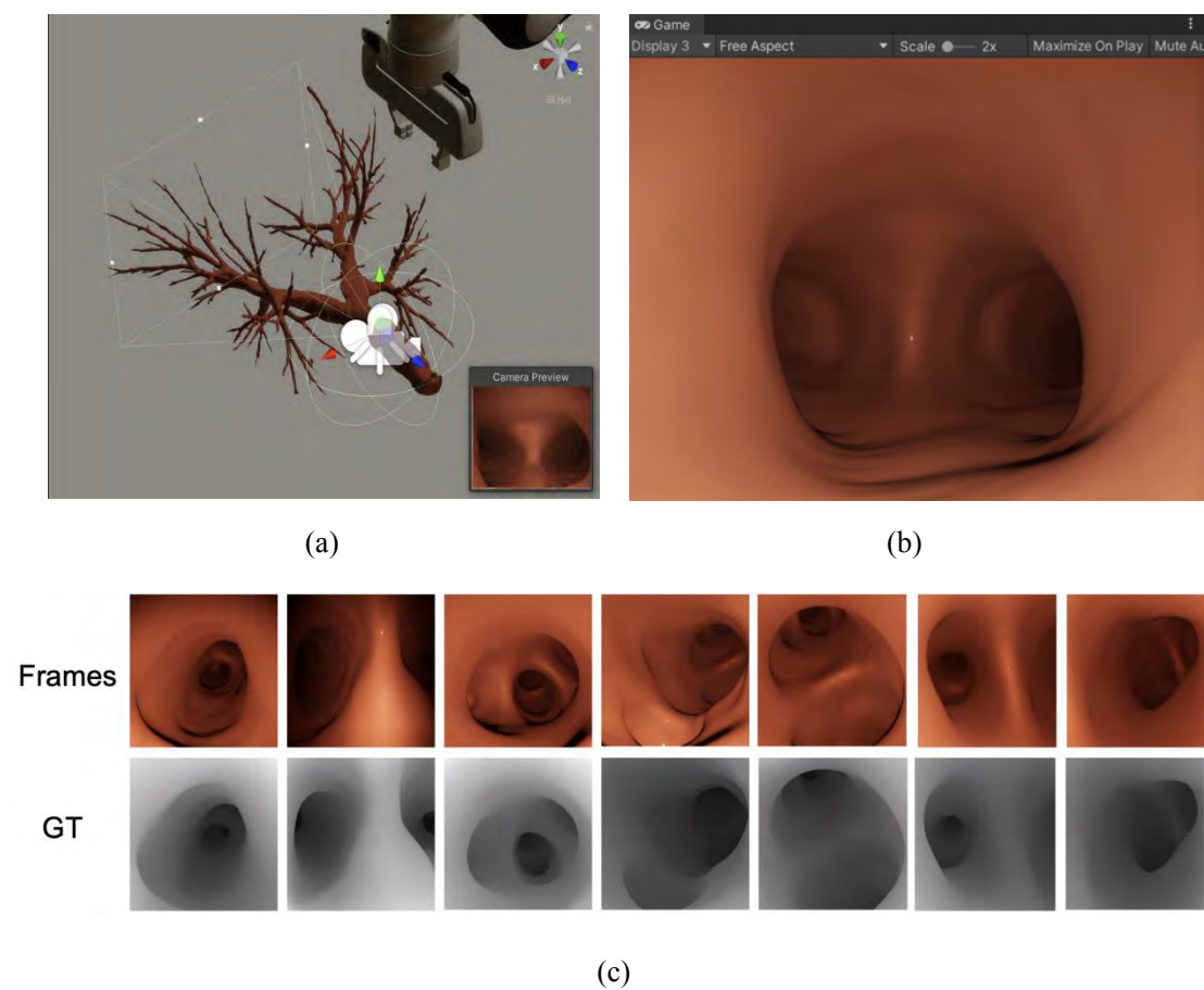
Fig. A1. Generation procedure of virtual image-depth pairs. (a) Segmented 3D airway mesh as the flythrough roadmap. (b) Camera simulation rendered with the bronchoscope's intrinsics. (c) Consecutive frames and their corresponding depth maps.
