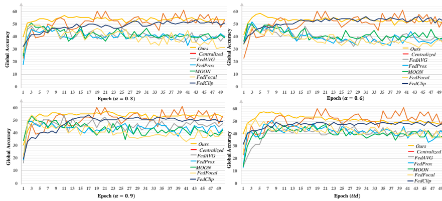
Fig. S1: Global testing ACC (%) using SC dataset for each round using our method and other comparable techniques.
