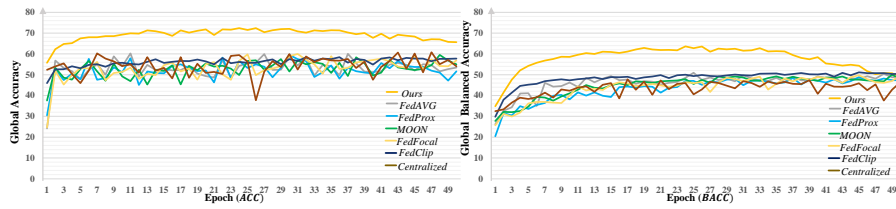
Fig. S2: Global testing accuracy (ACC%) and balanced accuracy (BACC%) using Real dataset for each round using our method and other comparable techniques.
