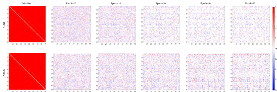
Fig. 2. Visualization results of the average brain networks/graphs of all subjects with different epochs. The first column is the initial brain network, which is a 90 \times 90 matrix with 0 on the diagonal and 1 elsewhere. The last column, Epoch=50, is the final brain network/graph after 50 epochs.
