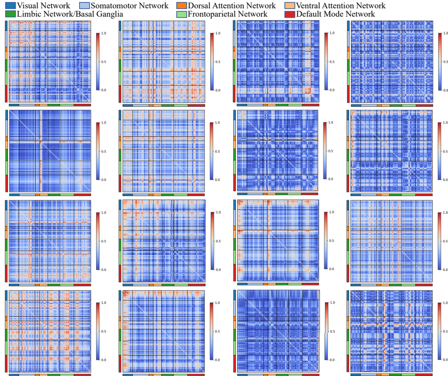
Fig.1. Discrepancy maps between ASD and NC groups of sixteen channels from learned function representations.
