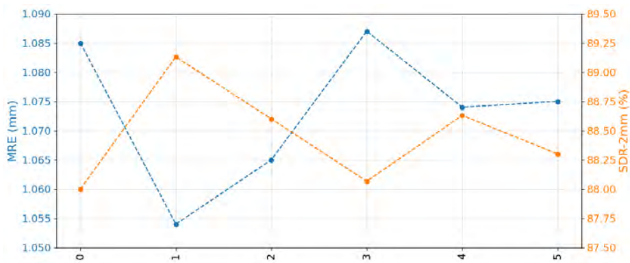
Fig. 1. Sensitivity analysis of \lambda_1 , with \lambda_2 fixed as 3.0
