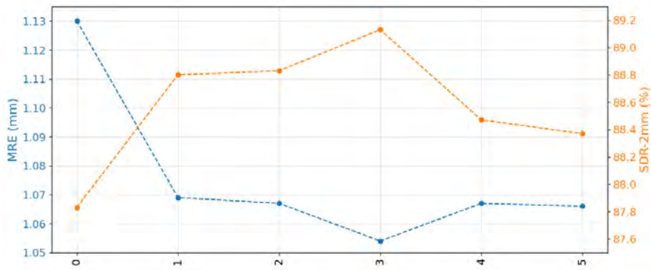
Fig. 2. Sensitivity analysis of \lambda_2 , with \lambda_1 fixed as 1.0
