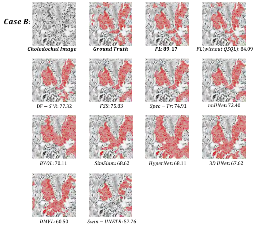
Fig. 2. Qualitative visualizations of the proposed FL and other state-of-the-art methods on the MDC dataset. Here we visualize another case.
