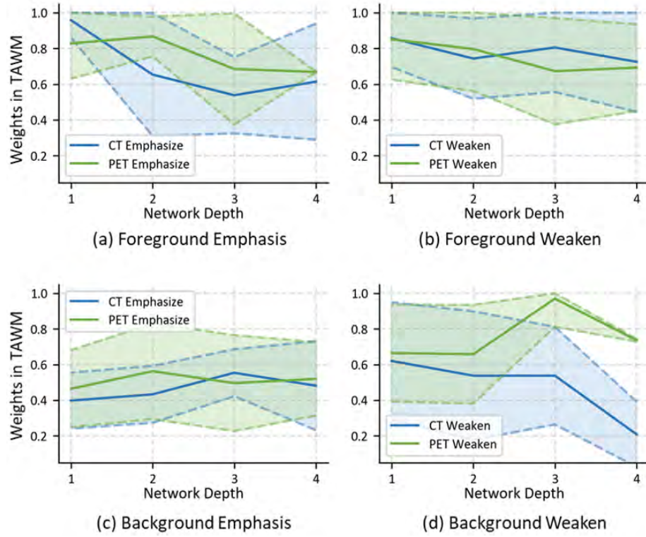
Fig. 2: Visualization of effect (%) of PET/CT in TAMW for reconstructing foreground and background at different depths.
