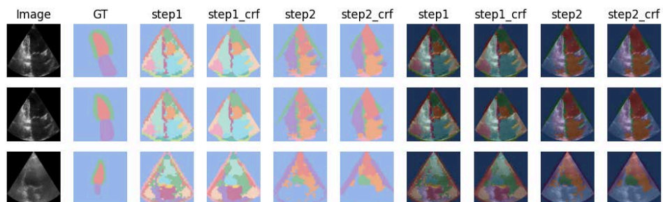
Fig. 3. Results for CAMUS
