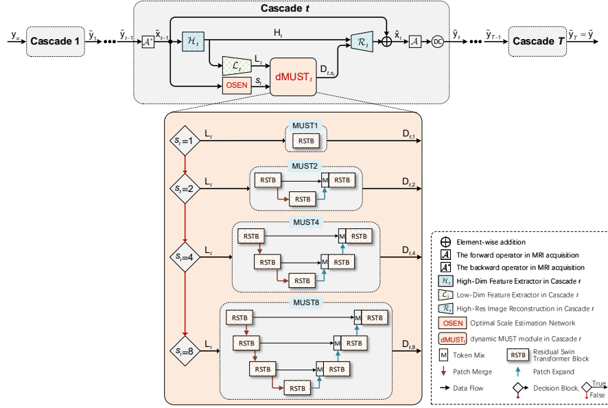
Fig. 1. Overview of the proposed dynamic Hybrid Unrolled Multi-Scale Network (dHUMUS-Net). The main module is the dMUST , i.e., the dynamic MUST (Multi-scale residual Swin Transformer) , which consists of several MUST -based branches (e.g., MUST1 , MUST2 and etc.), and will be dynamically constructed during training according to the repetition level of the input image estimated by OSEN .
